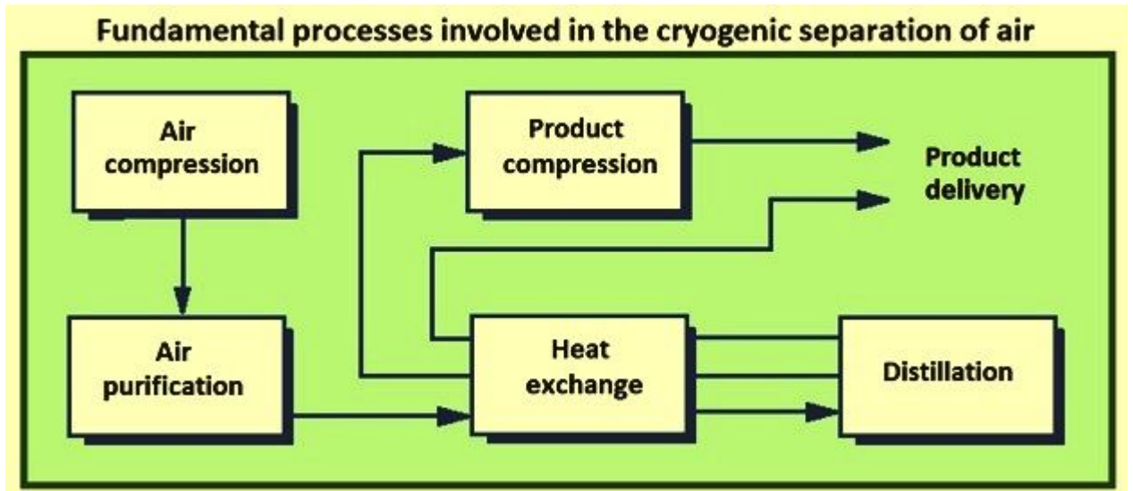
Figure 1 involves the basic process of cryogenic air separation
